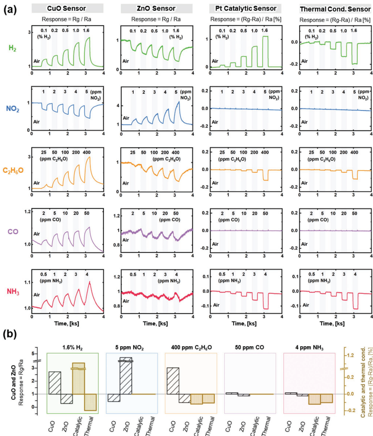
Figure 3. a). Dynamic responses of the chemiresistive sensors (CuO and ZnO) and the calorimetric sensors (catalytic combustion and thermal conductivity) to the exposure of risk-relevant concentrations of H 2 , NO 2 , C 2 H 6 O, CO, and NH 3 . b) Summary of the responses of the four sensors shown in part (a); the chemiresistive sensors have the same definition for their response (left axis), as do the calorimetric sensors (right axis).
