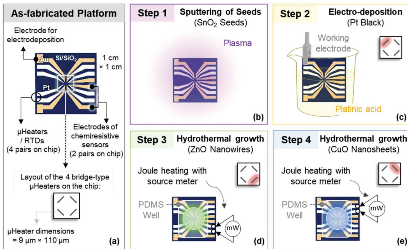
Figure 2. Overview of the fabrication process (integration of nanomaterials). a) top view of the chip. b) Step 1 consists of depositing the SnO 2 seed layer for eventual hydrothermal growth. c) The nanostructured Pt Black is synthesized via electrodeposition (the solution does not affect the seed layer). d) Local hydrothermal growth of ZnO nanowires using joule heating. e) Local hydrothermal growth of CuO nanosheets using joule heating. In steps 2–4, rinsing in acetone and ethanol is performed between steps and at the end.
