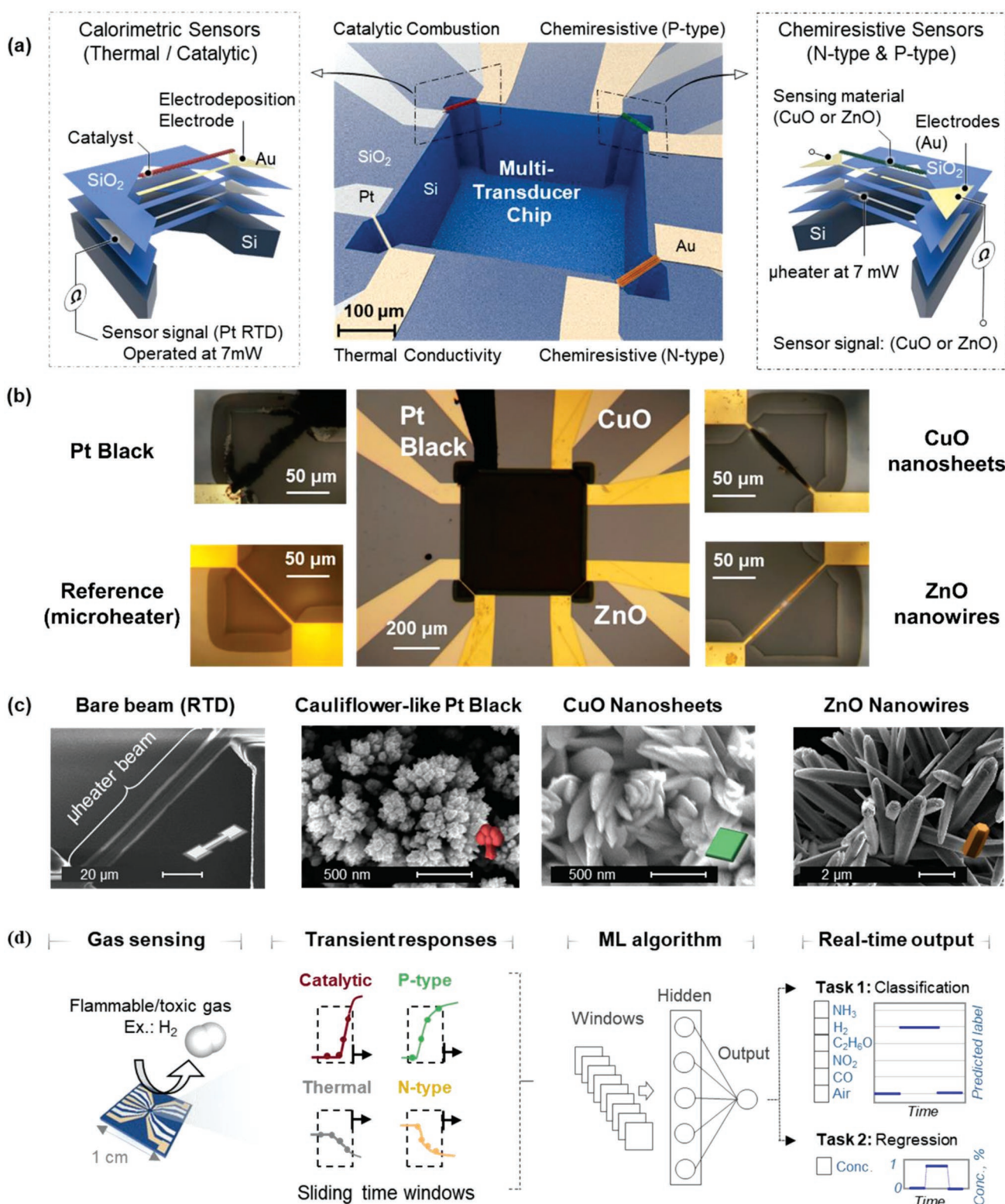
Figure 1. Overview of the multi-transduction gas sensor array for real-time gas sensing. a) Schematic representation of the constituent sensors in the array, including exploded views of the layers (sides). b) Optical microscope images of the fabricated array with all sensing materials synthesized. c) Scanning Electron Microscope images of the fabricated nanomaterials on their respective microheaters; the thermal conductivity sensor does not carry any nanomaterial and the bare microheater beam is shown here. d) Overview of the machine learning strategy, whereby transient responses are processed for real-time classification and regression.
