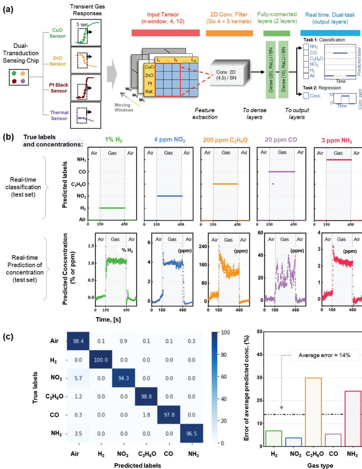
Figure 5. a) Data processing strategy to identify and quantify the concentrations of target gases in real-time using the four sensor signals. b) Real-time output (over time) of the classification task (top row) and regression task (bottom row). c) (left) Confusion matrix of the classification task showing high classification accuracy (>94%) for all gases, with an overall accuracy of 97.95%; (right) percent error of the regression task for each gas, showing an overall average error of 14 percent.
